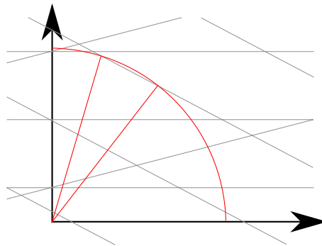
Fig. 10. In a rational multi-grid \mathcal{M}^{A, \mathbf{a}_i} a convexel can have four intersections with the locus of rotation of \mathbf{p} .
