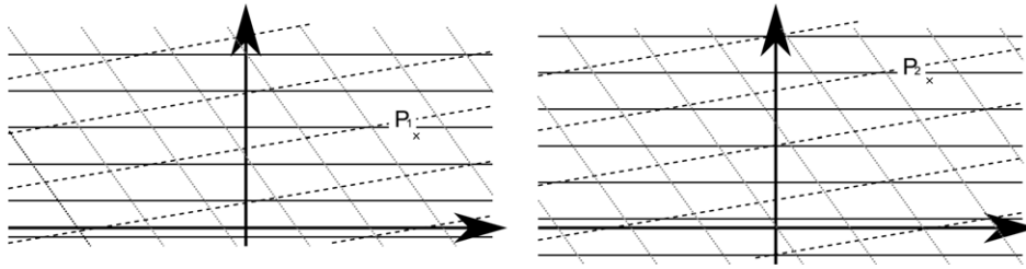
Fig. 5. Two multi-grids generated by a rotation axis but with two different points \mathbf{p}_1, \mathbf{p}_2 one of which is obtained by a translation of \pm(\mathbf{p}_1 - \mathbf{p}_2) from the other.
