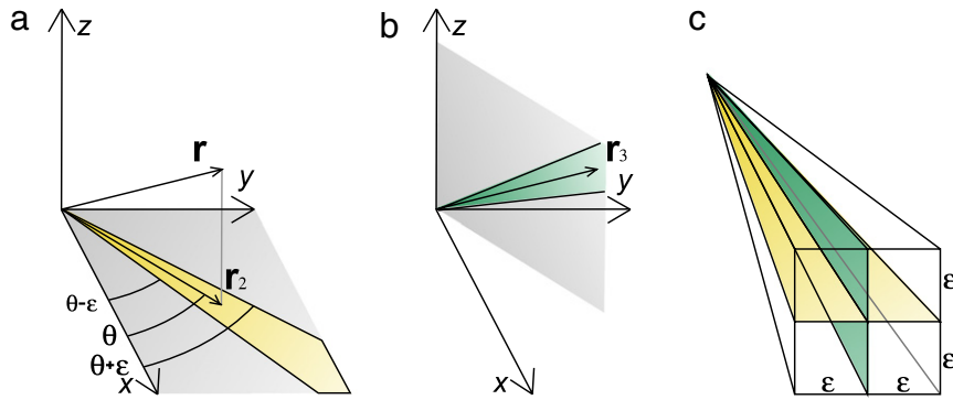
Fig. 9. Example of the approximation of a 3D vector using our method. (a) and (b) represent the projections of \mathbf{r} into \mathbf{r}_2 and \mathbf{r}_3 in 2D planes respectively. Each 2D convex cone in (a) and (b) is the admissible approximation for \mathbf{r}_2 and \mathbf{r}_3 regarding to \epsilon . (c) represents the square pyramid constructed from the two 2D convex cones that contains the set of admissible approximations for \mathbf{r} .
