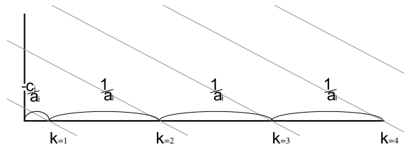
Fig. 3. Parallel lines of a set \mathcal{L}_i and geometric interpretation of their parameters.
