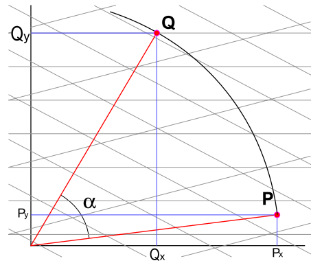
Fig. 8. A hinge angle \alpha for a point \mathbf{p} in a rational multi-grid.
