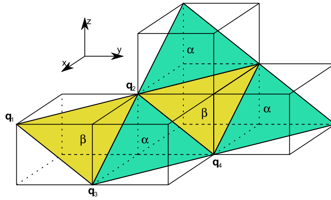
Fig. 6. A quadruple of grid points \{\mathbf{q}_1 = \mathbf{q}, \mathbf{q}_2 = (q_x + A_x, q_y + A_y, q_z)^\top, \mathbf{q}_3 = (q_x + A_x, q_y, q_z - A_z)^\top, \mathbf{q}_4 = (q_x + 2A_x, q_y + A_y, q_z - A_z)^\top\} forms two types of triangles, \alpha and \beta tiled in a multi-grid.
