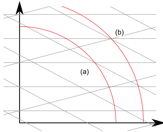
Fig. 7. The two impossible cases of intersection between a circle centered on a grid point and a rational multi-grid.
