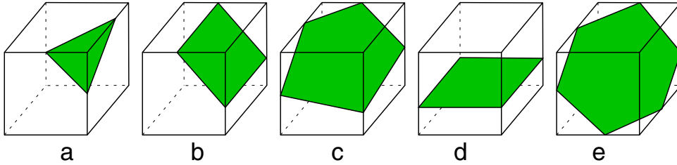
Fig. 4. The five different shapes of convexels, which are constructed as the intersections between a rotation plane and voxels [12].
